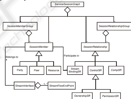
Figure 7: The Service Session Graph information model
