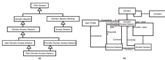
Figure 5: Important access session related information models:
