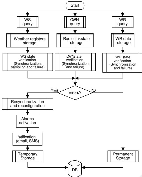
Figure 6: CS operations flowchart.
