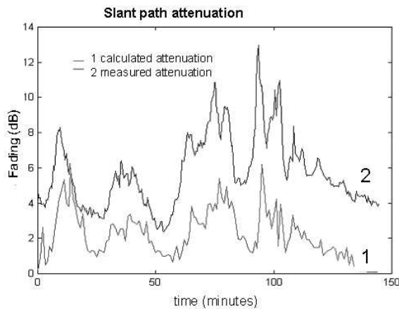
Figure 7: Comparison between measured and computed attenuation for the same radio link. Barcelona ITALSAT. 41^\circ elevation, 39.6 GHz.
