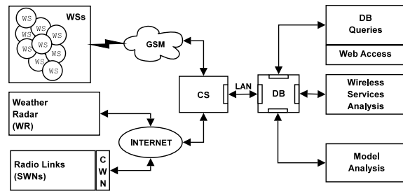
Figure 5: WAS architecture and database interfaces.
