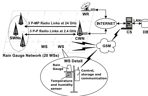
Figure 1: Weather station data Acquisition System (WAS) structure for the rain gauge network.
