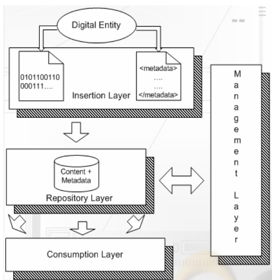
Figure 2: Digital Repository General Functional Model
