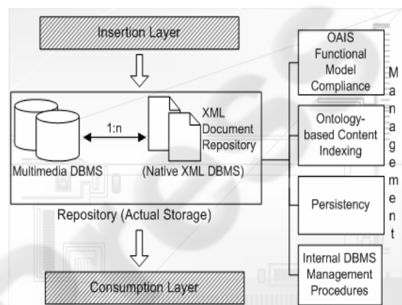
Figure 4: Digital Repository Functional Model in detail: The Repository (Actual Storage) and the Management Layers
