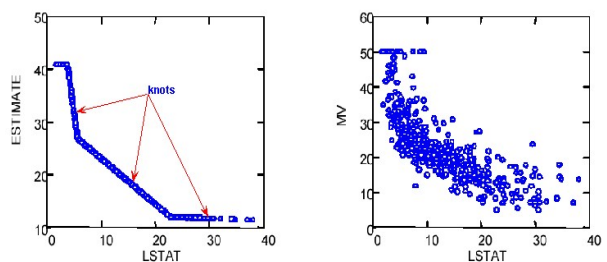
Figure 2: MARS data estimation using splines and knots
