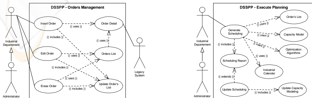
Figure 3: Use Case diagram for Orders Management package and for Execute Planning package.
