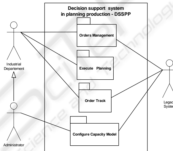
Figure 2: Use Case diagram for the proposal system.
