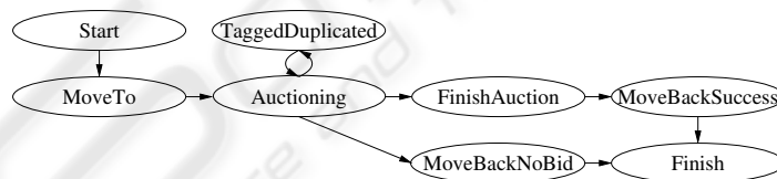
Fig. 2. Lifecycle of an auction agent
