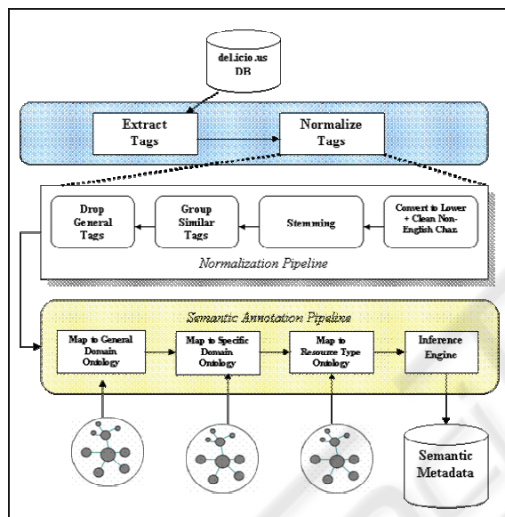
Figure 2: System Architecture of the 'FolksAnnotation' Tool.
