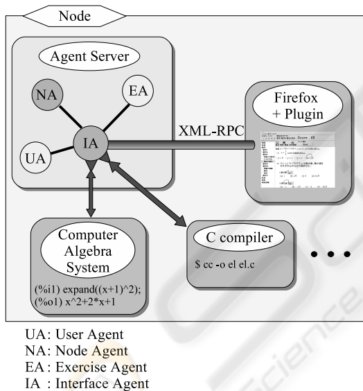
Figure 5: User and application interface and other components in a user studying node.
