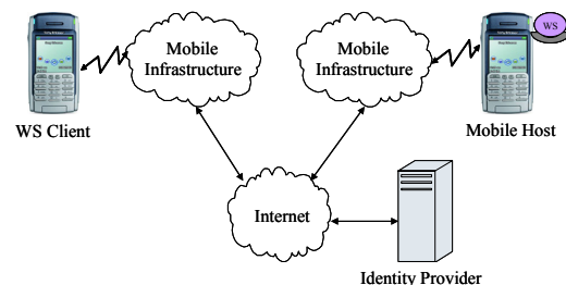
Figure 2: Mobile web service invocation test setup.
