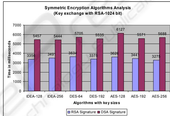
Figure 7: Performance latencies with signing on top of the encryption.
