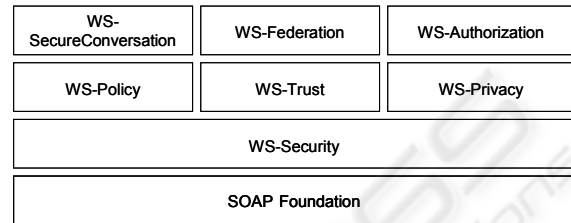
Figure 1: Web Service Security specifications.
