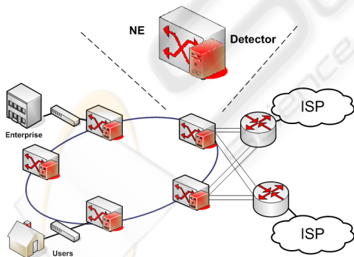
Figure 1: System architecture.
