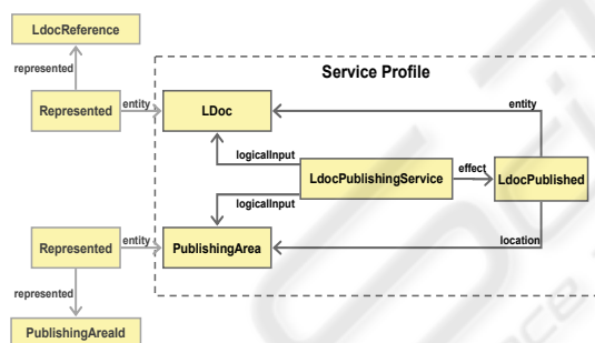
Figure 4: Example Service Profile.
