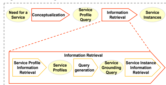
Figure 6: Semantic Service Retrieval Process.
