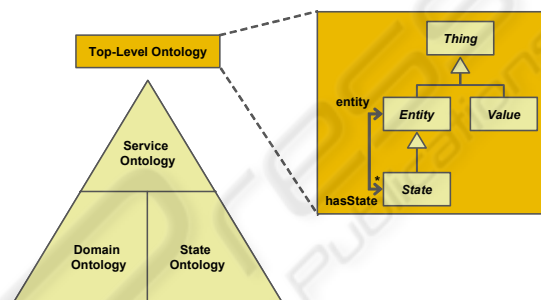
Figure 1: Service Description Ontologies.
