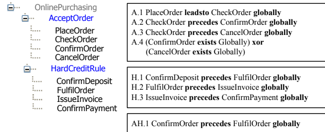
Fig. 6. Business Activities of the Online Purchase Example.
