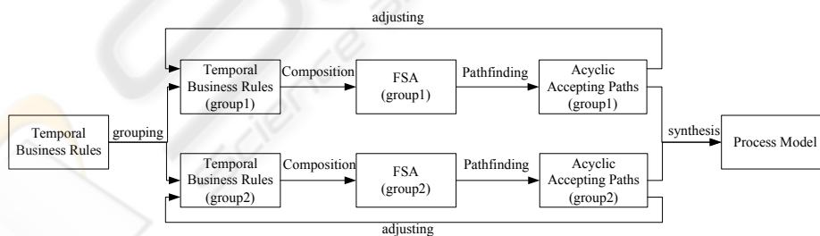
Fig. 5. Synthesis Process.
