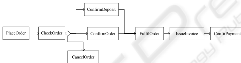
Fig. 10. A Possible Synthesized Process Model.
