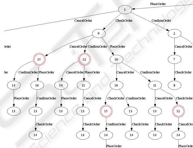
Fig. 9. Excerpt of the Path-Tree.
