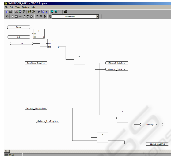
Figure 5: Example of the specification of a function in a bus using the ISaGRAF tool.
