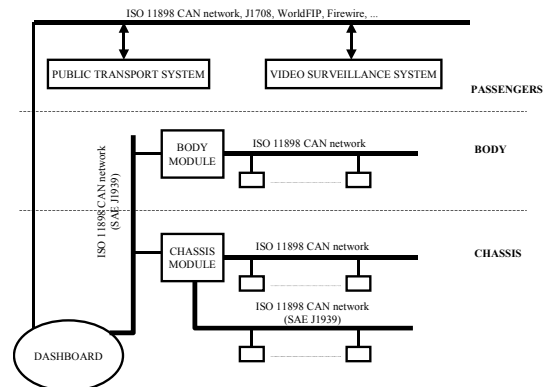
Figure 2: Levels in a typical city public transport bus.
