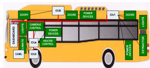
Figure 4: Structure of the networked control system onboard the bus.
