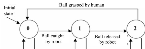
Figure 4: Finite state machine of the robot.
