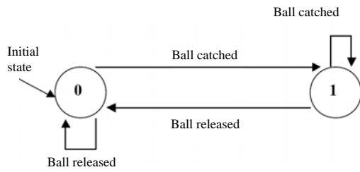
Figure 9: Finite state machine for the gripper.
