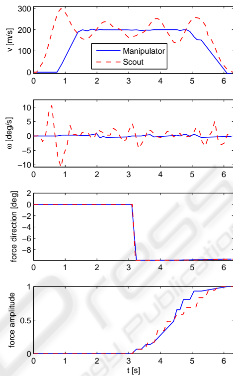
Figure 5: Velocities and force feedback recorded during two robot collision experiment.
