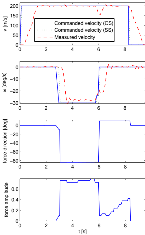
Figure 4: One robot experiment: driving around a corner.
