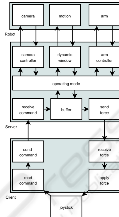
Figure 2: Event-Based Action Synchronization between client and server control modules.
