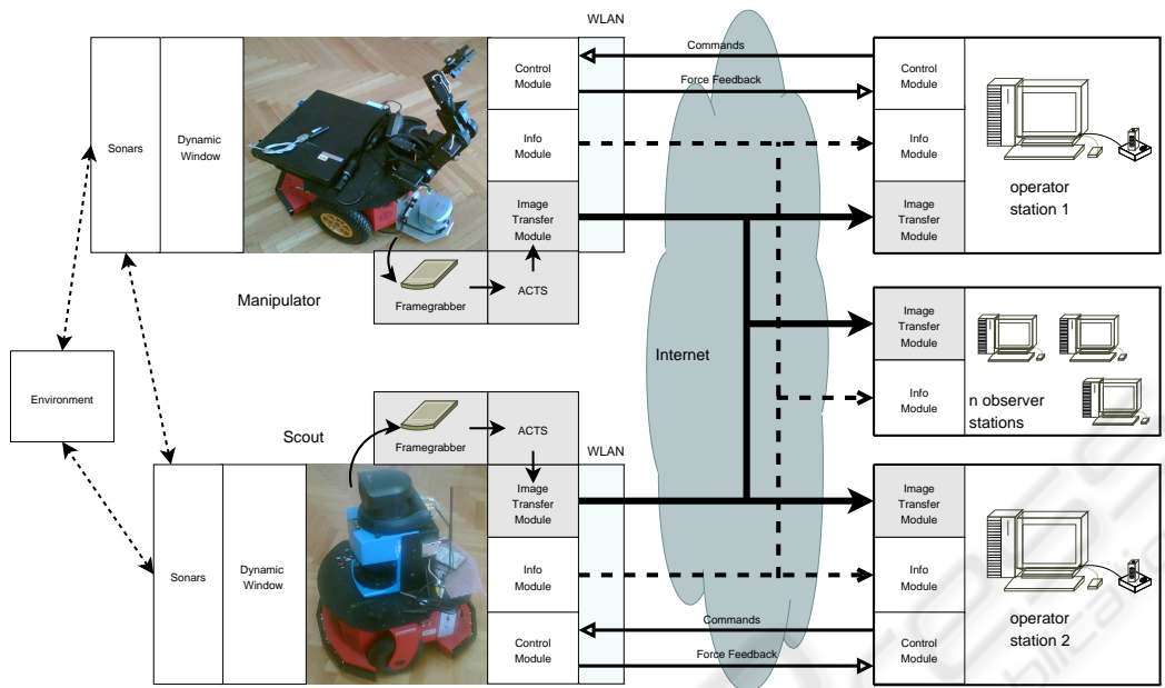
Figure 1: Schematic overview of the teleoperation system.
