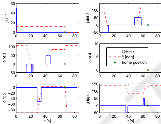
Figure 7: Motion of the robot arm joint angles during the two robots experiment.
