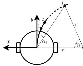
Figure 3: Trajectory of a robot is described as a circular arc.
