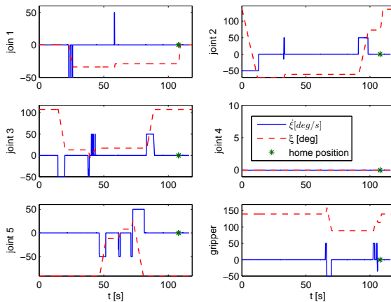
Figure 6: Motion of the robot arm joint angles during the one experiment.
