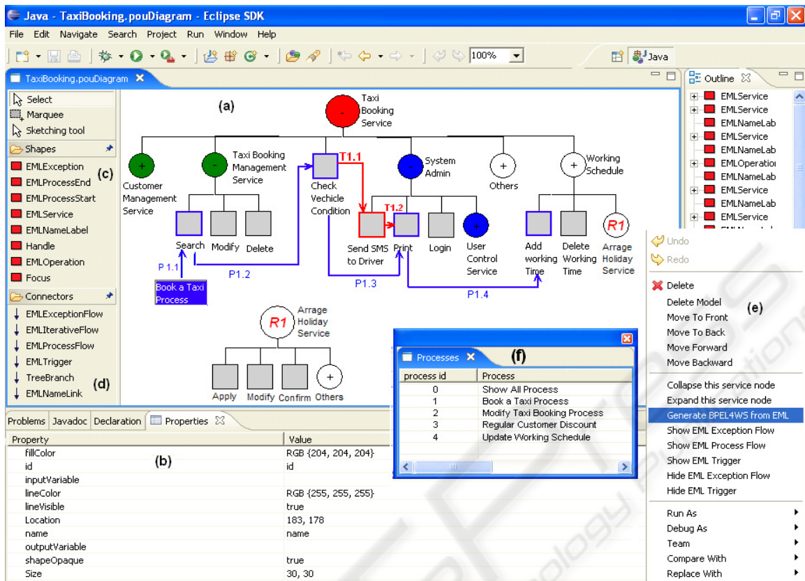
Figure 1: Using MaramaEML to Create Book a Taxi Process.
