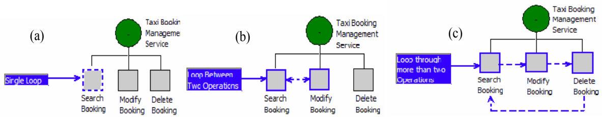
Figure 2: Different Loops in EML.
