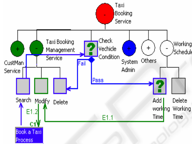
Figure 3: Exception Handler.
