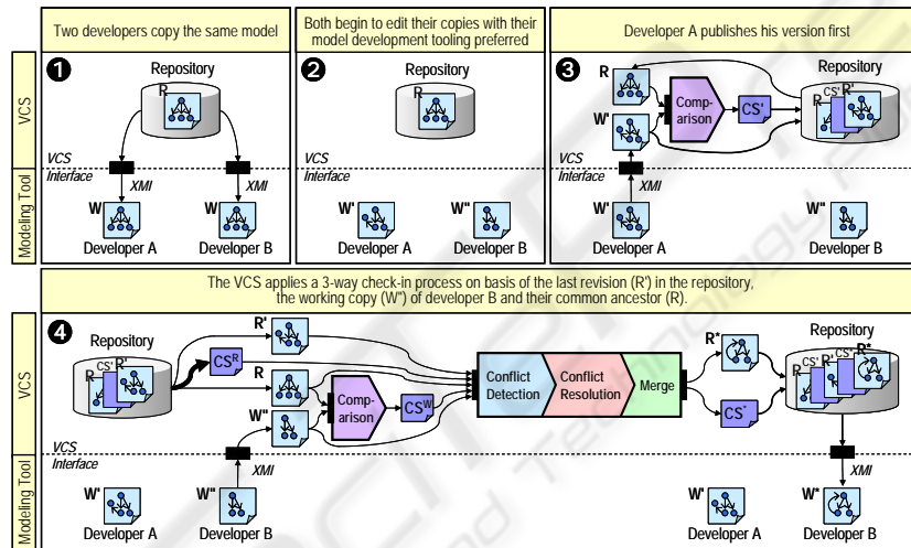
Fig. 4. Workflow scenario of the proposed approach.
