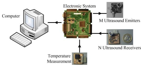
Figure 7: Precision positioning block diagram.
