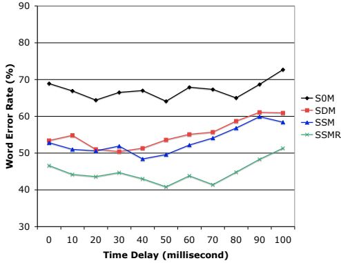
Figure 7: Word Error Rate on Spectral+Temporal Features.
