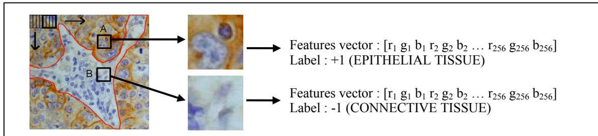
Figure 6: Generation of the features vectors for SVM training. A N \times N square window is horizontally and vertically shifted on the sample, thus covering the entire surface of the image. For each shift a features vector is generated with RGB values of 256 equally spaced pixels, as for Window A and Window B. Epithelial instances are labelled with a +1, connective instances with a -1.
