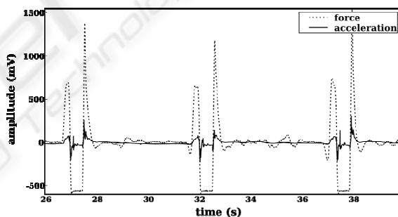
Figure 3: Acceleration and force curves of a series of 3 vertical jumps.
