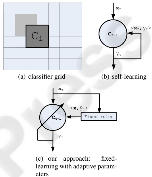
Figure 2: (a) The background model is formed by a highly overlapping grid of classifiers. Updating the former approach (Grabner et al., 2006) uses self-learning (b). Our proposed method (c) does not directly take the classifier responds y_t = C_{t-1}(x_t) into account and thus do not suffer from the drifting problem.
