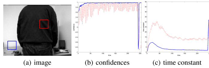
Figure 4: Confidences (b) and estimated time-constants (c) for two different patches (a) over time. As can be seen, the blue patches covers a non-dynamic scene, reliably detects the intruder and immediately recovers its state. The second patch (red) has to handle dynamic flickering background. Hence, the time-constant also stabilizes around a higher value than for the blue patch. However, when the scene changed dramatically the time-constant raised very high making it very difficult for the intruded object to fade into the background.
