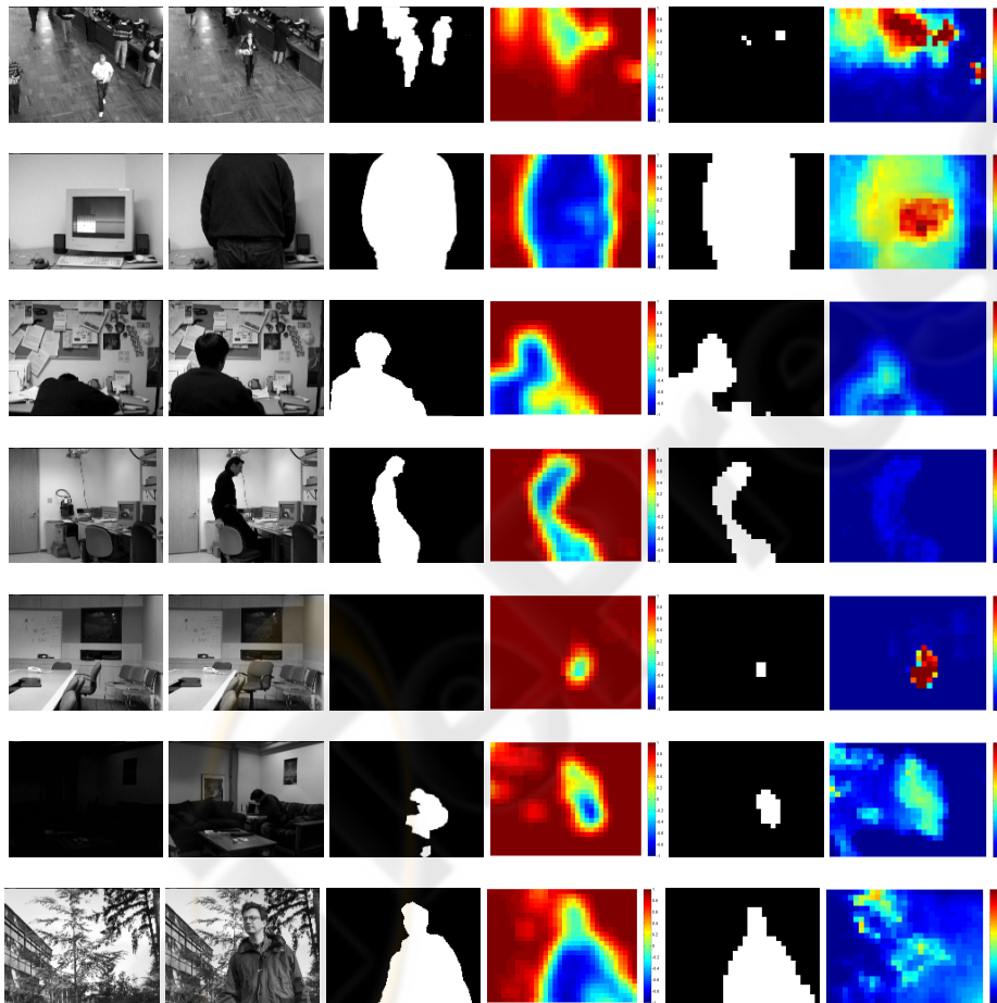
Figure 5: Detection results of our method for the test sequences presented in (Toyama et al., 1999). The first column shows the initial frame of each sequence, second column the test frame and the third column the hand segmented ground truth. In the last three columns our results (the real valued confidence map, a binary segmentation achieved by zero thresholding as well as the time constants) are depicted. Note that the performance could be easily increased by analyzing the confidences more closely.
