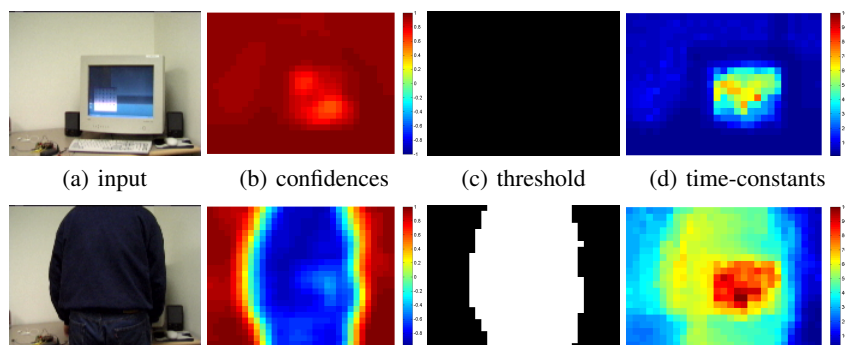
Figure 3: The first row depicts the test scene after t = 100 and the second row at t = 251 , respectively. The second column shows the yielded confidences. As we assume the flickering monitor to be background, the confidences are quite high. In order to achieve such results our control system autonomously sets the \Delta t in the flickering area higher than in the non-dynamic rest of the scene.
