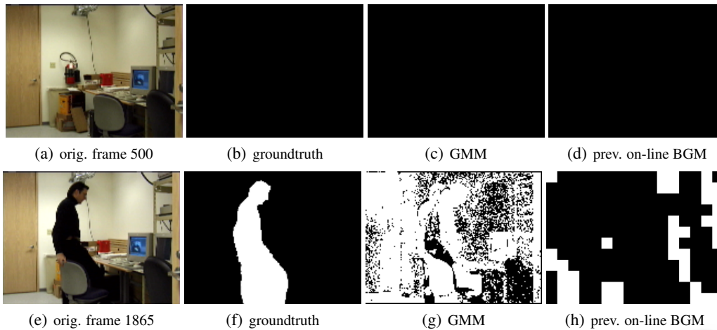
Figure 1: Comparison of BGM based on Gaussian Mixture Models (GMM) (Stauffer and Grimson, 1999) and an on-line classifier grid (Grabner et al., 2006) at a challenging Wallflower scene (Toyama et al., 1999). The first row depicts the results after 500 frames, where both adaptive approaches still perform well. From frame 829 to 1844 the lights are switched off. The second line depicts the result at frame 1865. As can be seen, both approaches fail because the GMM does not take neighboring pixels into account and the on-line classifier drifts away due to false updates during the lights-off phase.
