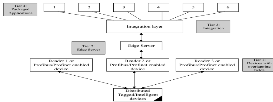
Figure 5: 4-Tier Reference Architecture.
