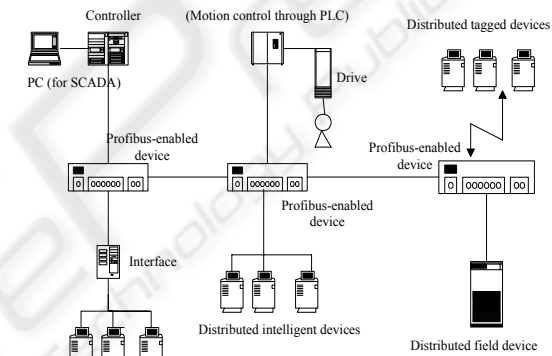
Figure 1: Typical Process Control Network.
