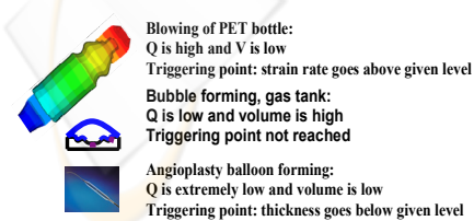
Figure 13: Development of volume flow Q and volume V for some thermoforming processes.
