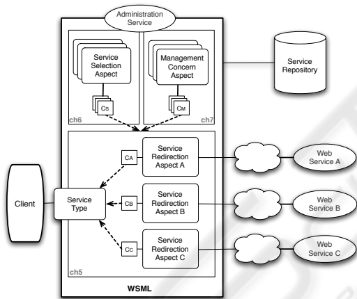
Figure 2: WSML Architecture.
