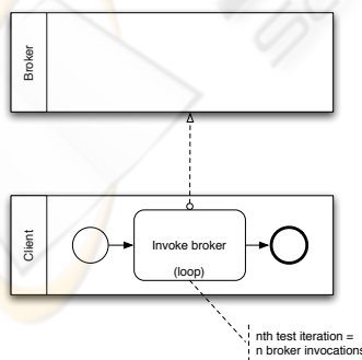
Figure 4: Client behavior.
