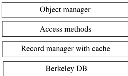
Figure 1: Storage manager.
