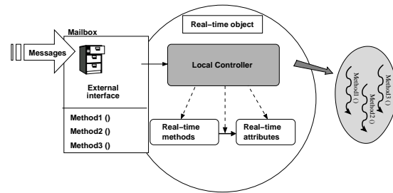
Figure 1: Schema of the Real-time object.
