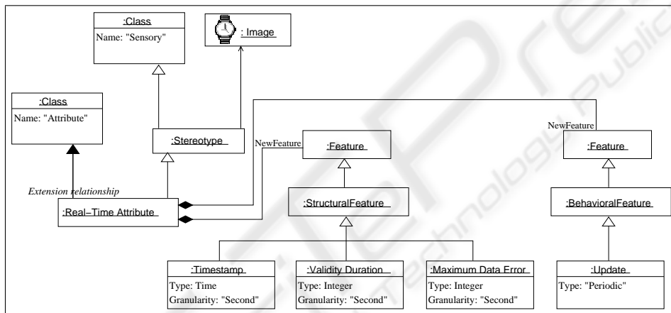
Figure 4: Abstract syntax of the «Sensory» stereotype.
