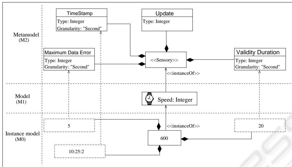
Figure 5: Instance Model of the <<Sensory>> stereotype.
