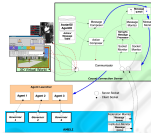
Figure 4: Causal Connection Server Architecture.
