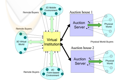
Figure 2: The system architecture example.
