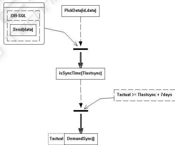
Figure 3: Behaviour diagram for Reminder caste.
