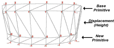
Figure 6: Cone-like shape created inside the geometry-shader stage.
