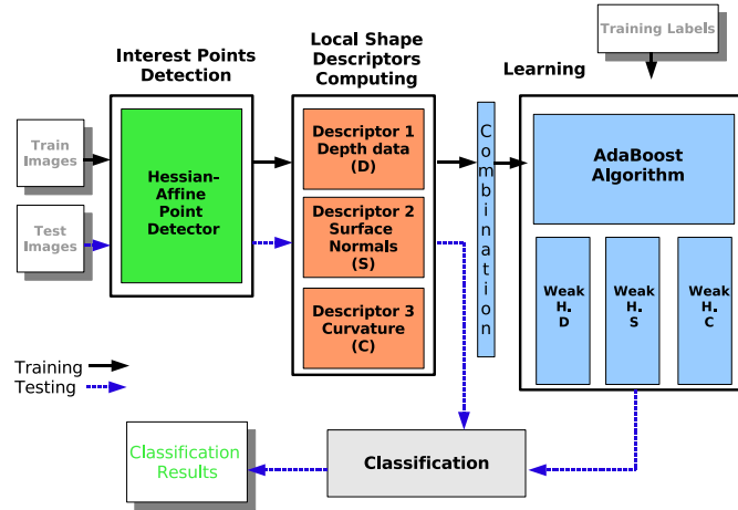
Figure 2: The proposed generic 3D object recognition model.
