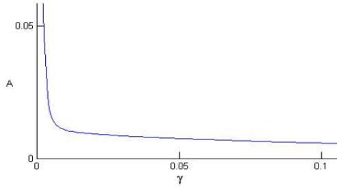
Figure 9: The function A(\gamma) for Fig. 8a.
