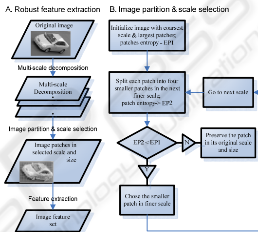
Figure 1: Robust feature extraction.
