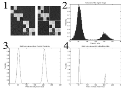
Figure 4: Comparison of FDA in simulation image.
