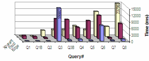
Figure 4: Execution Time over DBLP Database.
