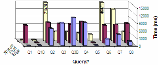
Figure 6: Execution Time over TREEBANK Database.
