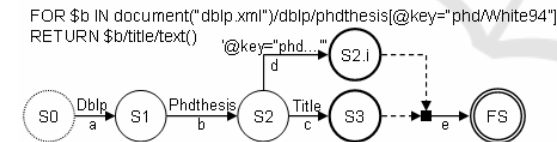
Figure 3: An XQuery Example and its FSM Execution Plan.
