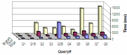
Figure 5: Execution Time over XMARK Database.
