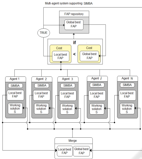
Figure 1: Multi-agent system supporting SIMBA.
