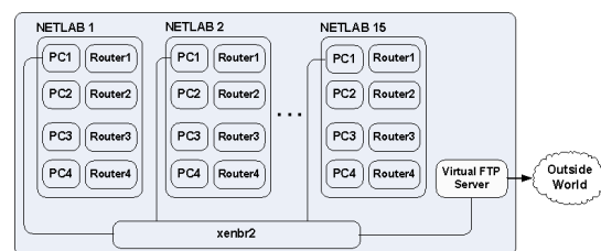
Figure 12: Configuration with Virtual FTP Server.
