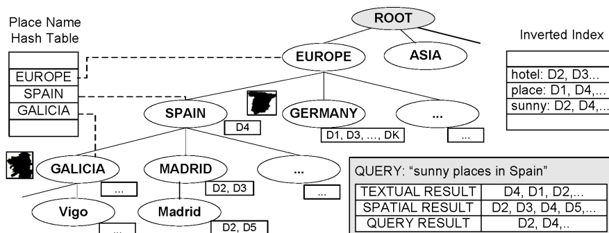
Figure 2: Index structure.
