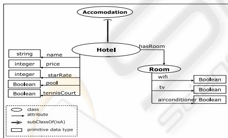
Figure 3: Tourism Ontology Concepts.
