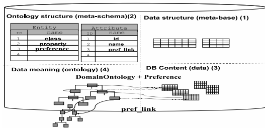
Figure 1: The OntoDB four parts architecture.
