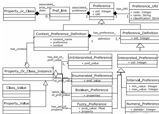
Figure 2: Our Model for Preferences.
