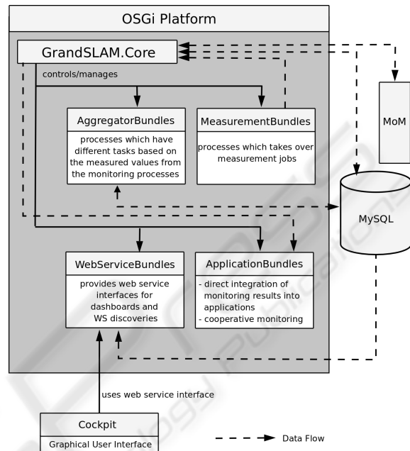
Figure 1: OSGi-based architecture of Grand SLAM.
