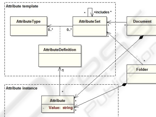
Figure 5: The “Dynamic Attributes” mechanism.
