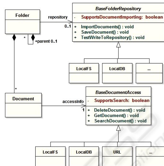
Figure 8: Support for multiple kinds of repositories.
