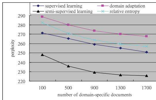
Figure 1: Perplexity test results of different learning approaches with different size of D^I .
