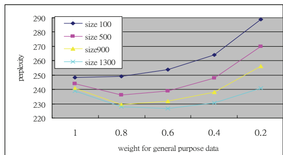
Figure 2: Perplexity test results of different models obtained with different size of D' and different \lambda .
