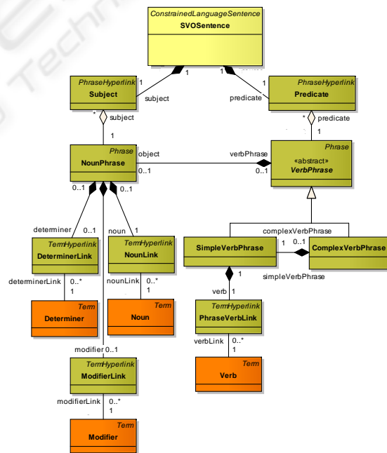
Figure 1: The structure of SVO-Sentences in RSL.
