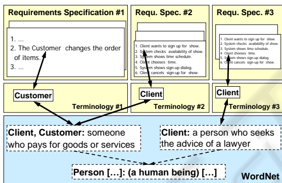
Figure 2: Relations between Requirements Specification, Terminology and WordNet.
