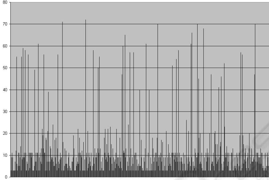
Figure 3: Assertion distribution among partitions in node 1 (3 nodes).
