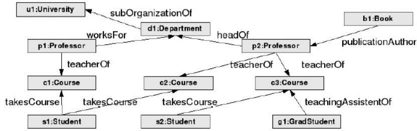
Figure 1: Guiding Example: ABox \mathcal{A}_{EX} for ontology O_{EX} .
