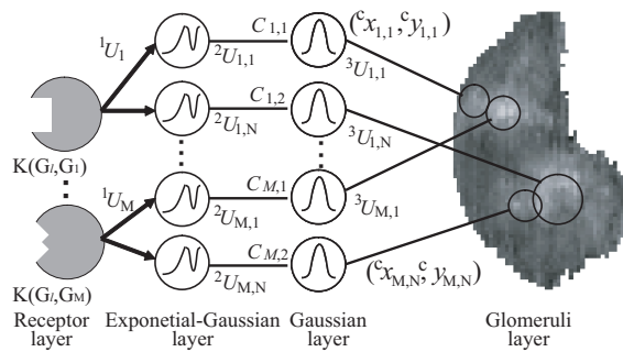
Figure 3: The proposed model for the olfactory system of rats.
