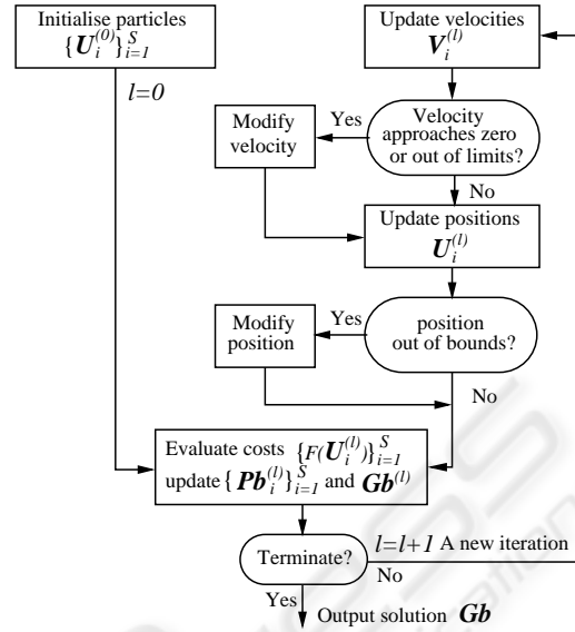
Figure 1: Flowchart of the PSO algorithm.
