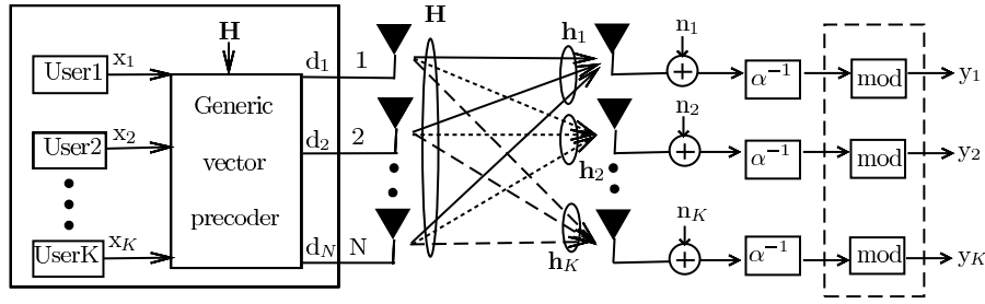
Figure 6: MUT-aided MIMO system with nonlinear VP, where the BS employs N transmit antennas to communicate with K MSs each equipped with a modulo device.
