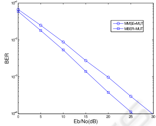
Figure 3: BER performance of the PSO-aided linear MBER-MUT design for the 4 \times 4 MIMO system, in comparison with the benchmark MMSE-MUT.
