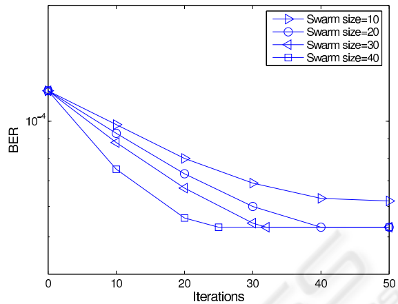
Figure 9: Convergence of the PSO-aided MBER generalised VP scheme with different swarm sizes for the 2 \times 4 MIMO system given SNR = 25 dB.
