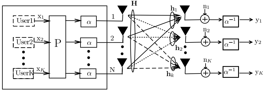
Figure 2: MUT-aided MIMO system with linear precoding, where the BS employs N transmit antennas to communicate with K single-antenna mobile devices.
