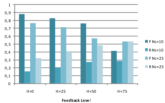
Figure 5: Comparison of the P and R values obtained when Ns=10 and Ns=25 and for the four degrees of historical information for the tourism domain.
