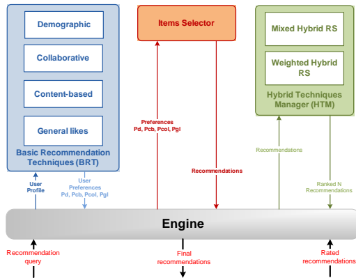
Figure 3: GRSK Architecture.
