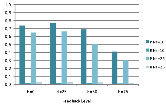
Figure 6: Comparison of the P and R values obtained when Ns=10 and Ns=25 and for the four degrees of historical information for the movies domain.
