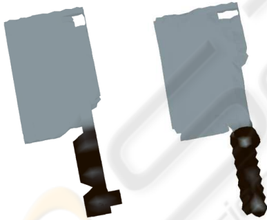
Figure 7: The non data-driven (left) and the data-driven (right) intermediate meshes for the cleaver model at 2 bpv.
