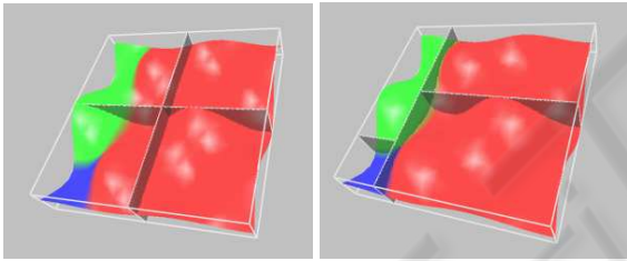
Figure 2: Illustration of the first two cuts (4 cells) of a simple model for the non data-driven (left) and the data-driven (right) versions of the algorithm. The non data-driven cuts subdivide the parent cell into 2 equal children cells, while the data-driven cuts follow the color borders.
