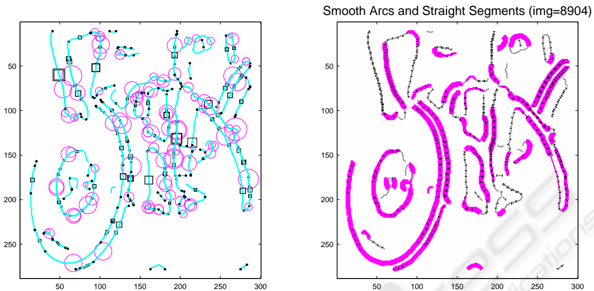
Figure 1: Decomposition output for an image (wheel chair from Caltech-101 collection). Left: Contour endpoints are marked as small black circles; squares and circles denote straight and curved segments respectively (their size reflects segment length - not curvature). Overlapping circles result from the global-to-local identification of elementary segments. Right: Smooth arcs (thick gray [magenta]) and straight segments (thick stippled) after application of a simple smoothness criterion to individual contours.
