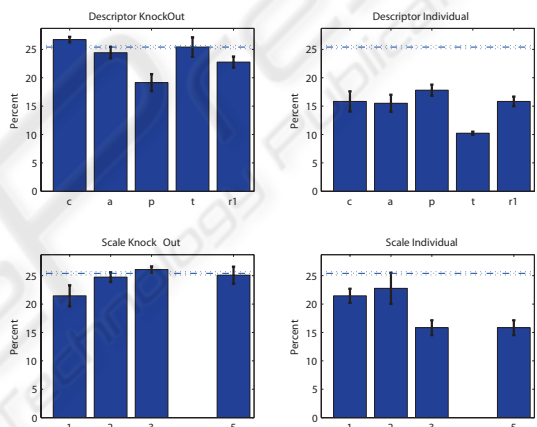
Figure 4: Performance (correct categorization) for 2 and 5 training images (a and b) for descriptor knock-out (upper left), individual descriptors (upper right), spatial scale knock-out (lower left) and individual scale (lower right). Note the performance increase for individual descriptors for 5 training images (compare upper right graph of a and b). Stippled horizontal line: total performance; dotted lines and error bars: standard deviation of crossfolds. c: contours; a: areas; p: polygons; t: textures; r1: regions.
