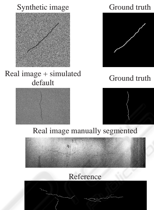
Figure 7: Tested images.
