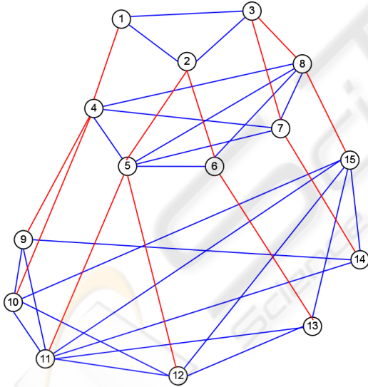
Figure 2: Illustration of the HCRF model architecture. The number of the nodes correspond to the regions in Figure 1. The blue edges between the nodes represent the neighborhoods at one scale, the red edges represent the hierarchical relation between regions.
